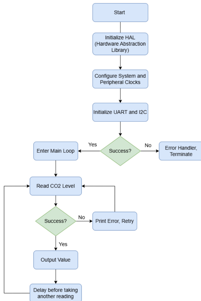
Figure 33: SCD41 CO2 Sensor Flowchart
