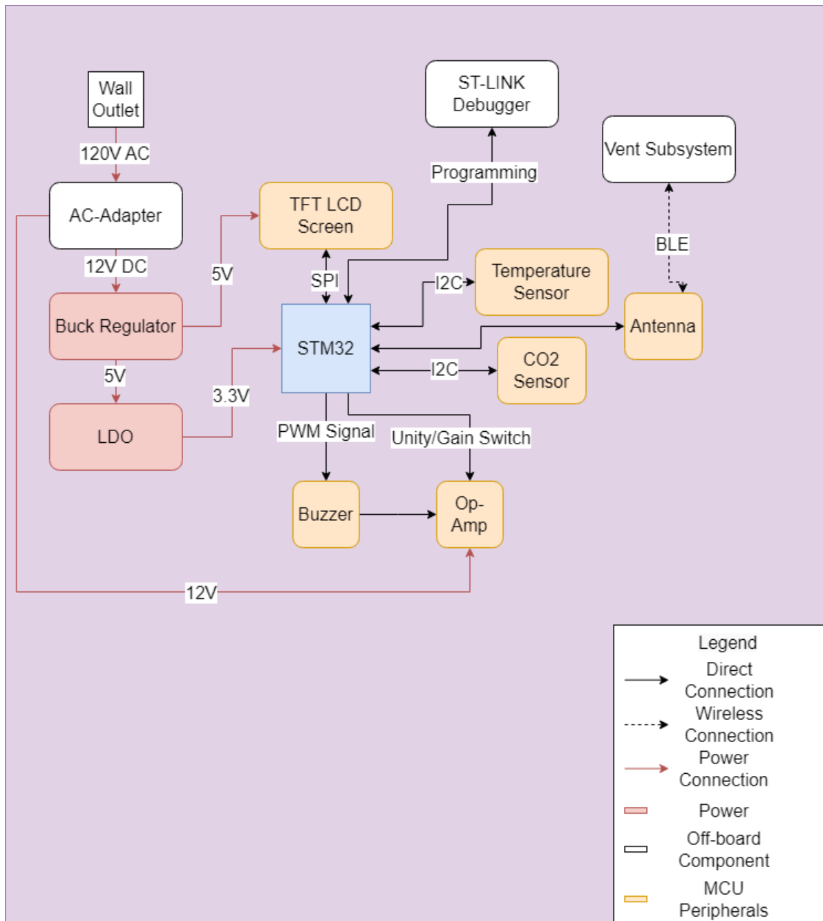
Figure 12: Hardware Block Diagram for Control Unit
