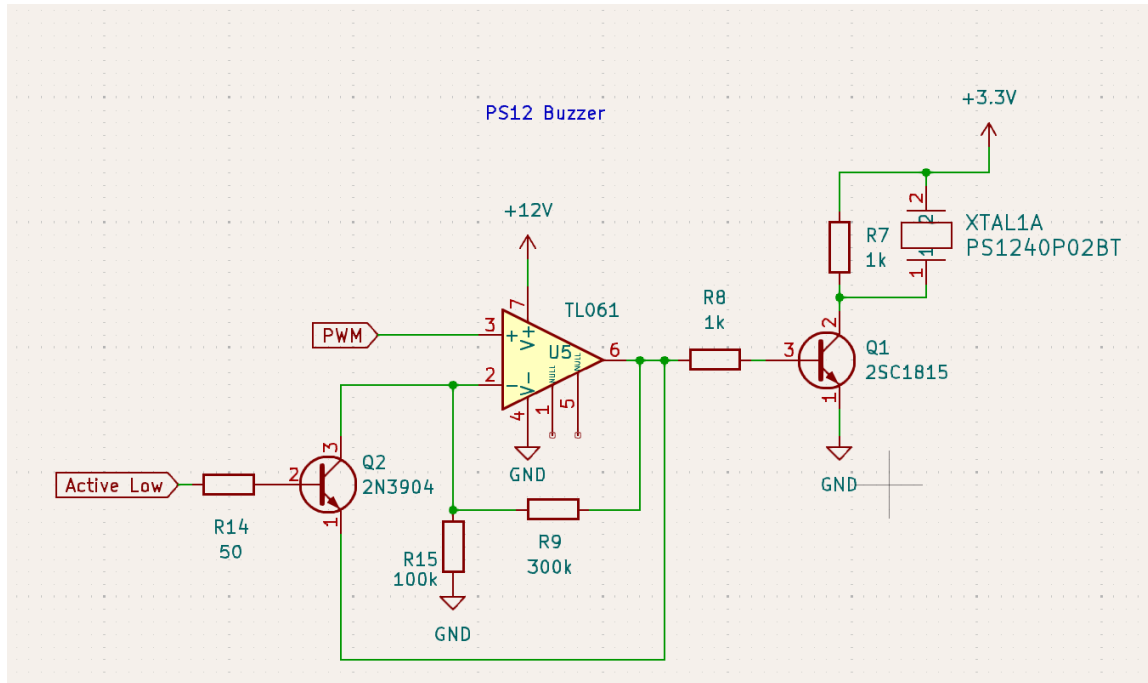
Figure 17: Buzzer Schematic
