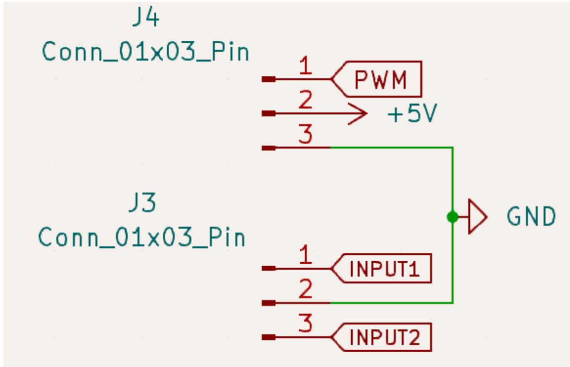
Figure 23: Vent Interaction Subsystem PCB Overall Schematic
