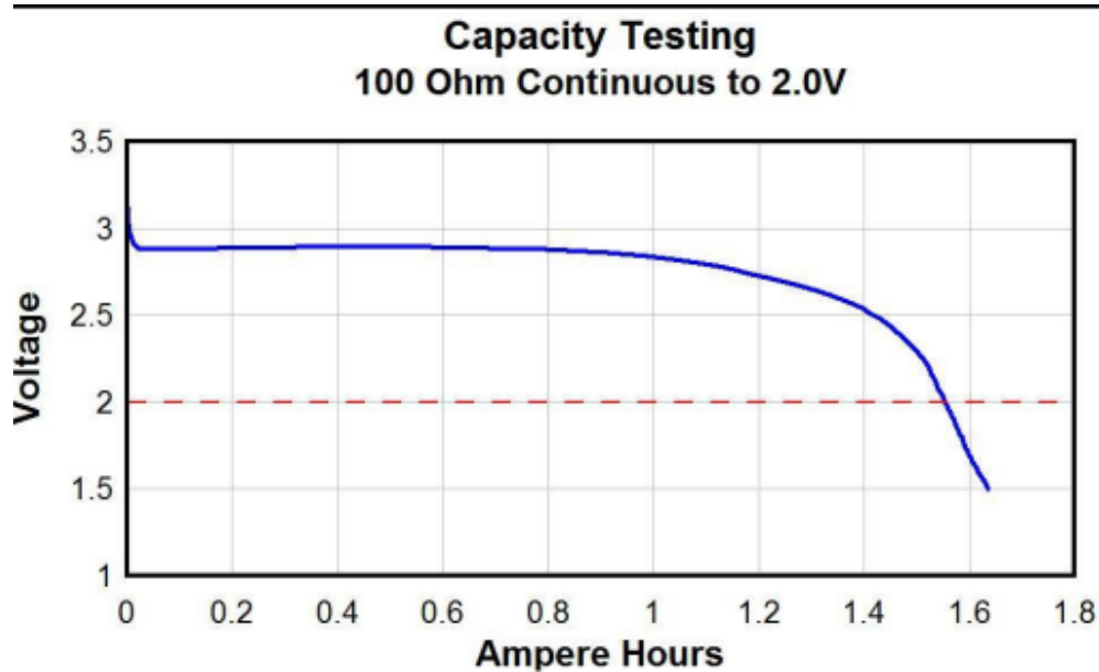
Figure 10: Duracell CR123 battery discharge voltage over capacity [69].
