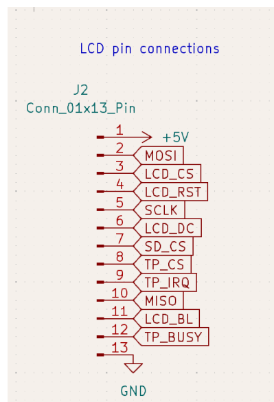
Figure 14: LCD Pin connections
