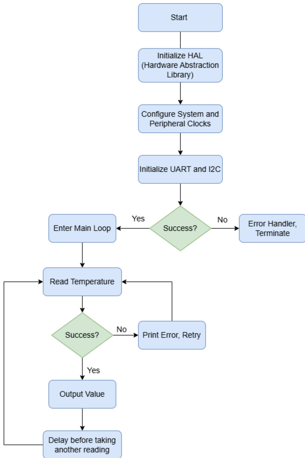
Figure 32: TMP102 Temperature Sensor Flowchart
