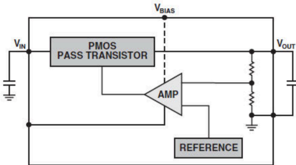
Figure 9: Basic LDO Block Diagram [61].
