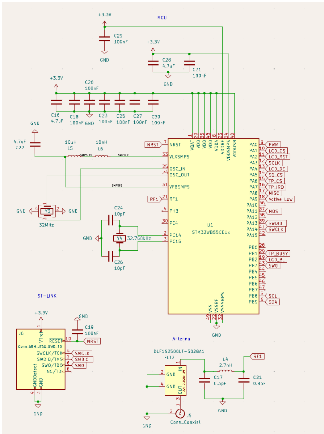
Figure 13: Control Unit MCU Isolated Schematic
