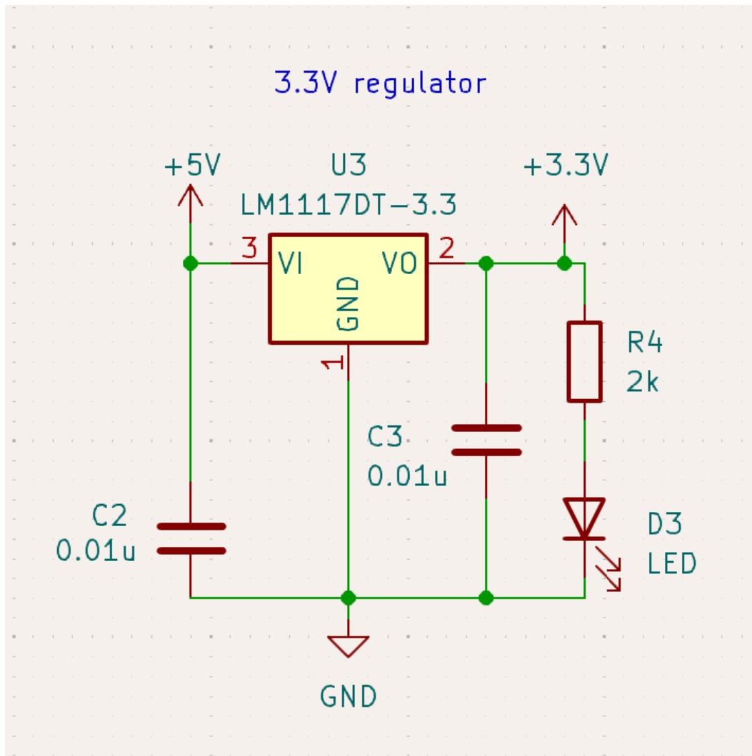
Figure 20: LDO Regulator for MCU
