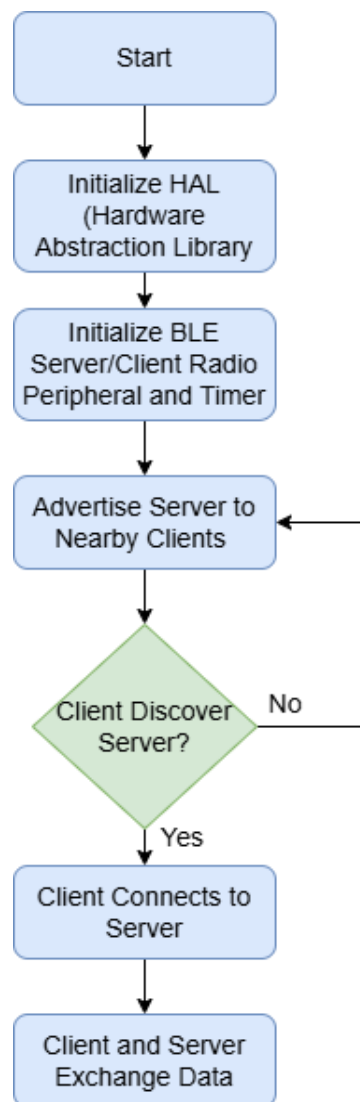
Figure 34: BLE Testing Flowchart
