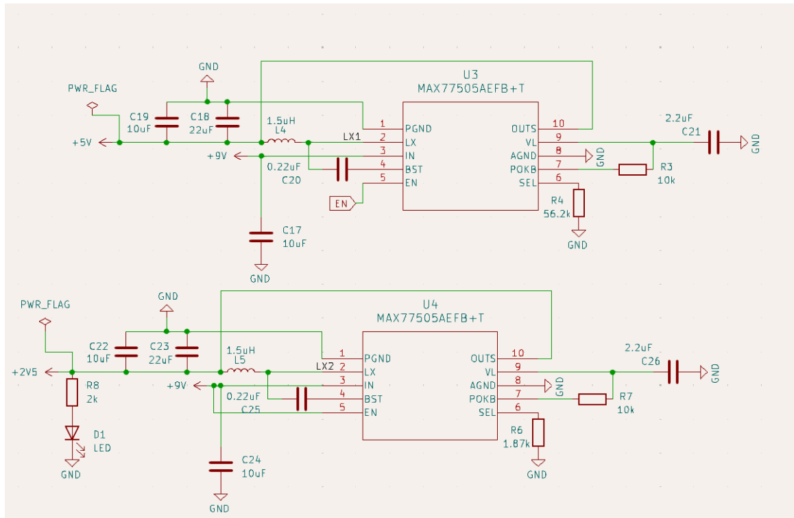
Figure 29: Buck-Regulator 2.5V and 5V Rail
