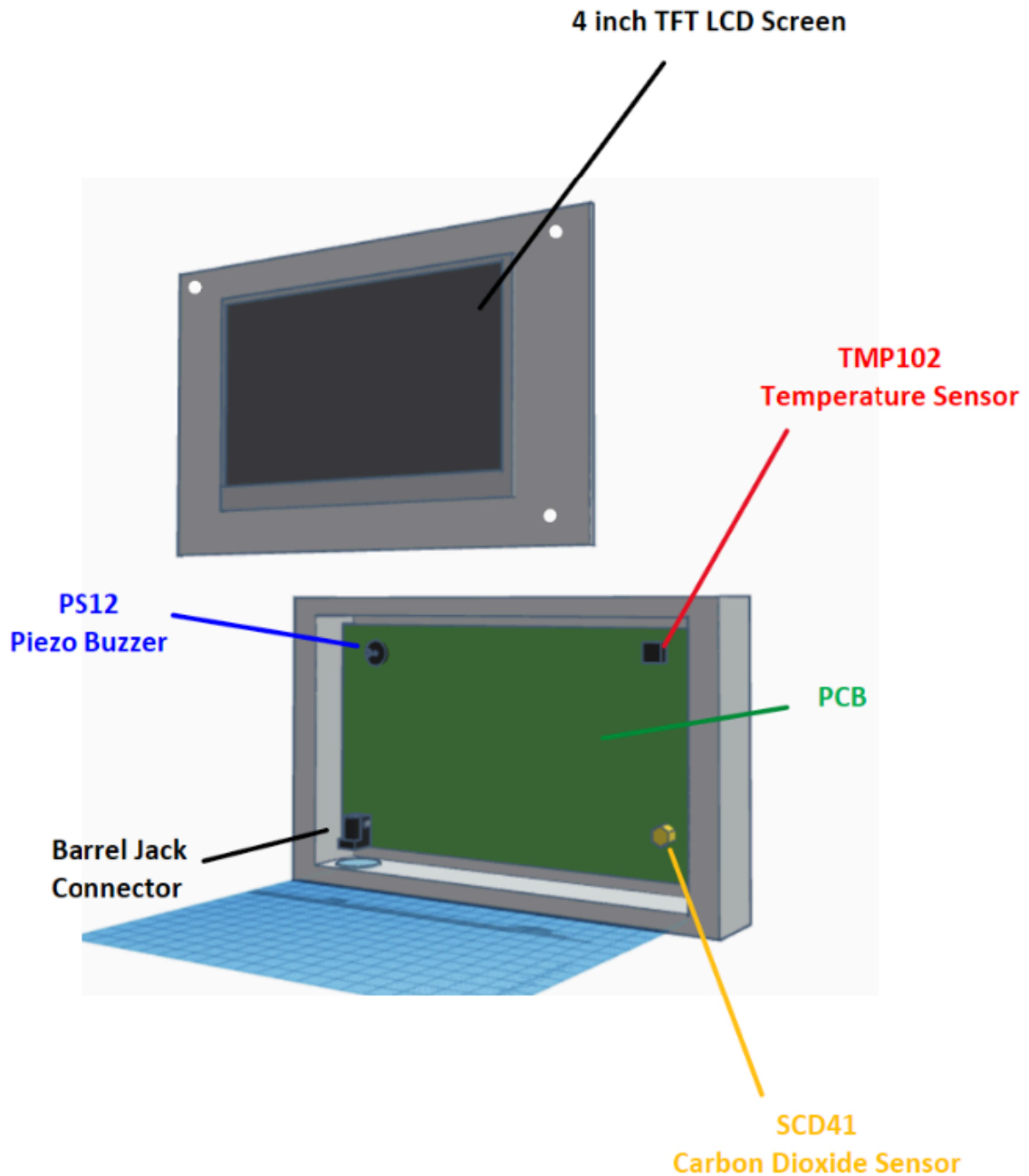
Figure 43: Prototype design for Control Unit
