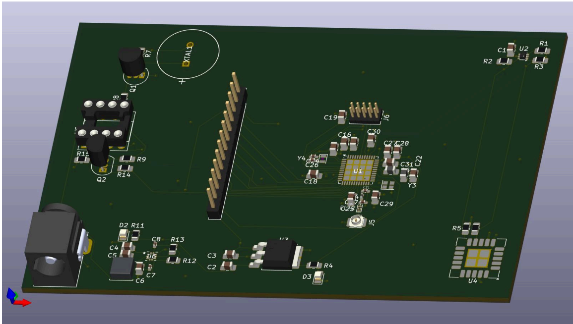
Figure 40: 3D Model of Control Unit PCB
