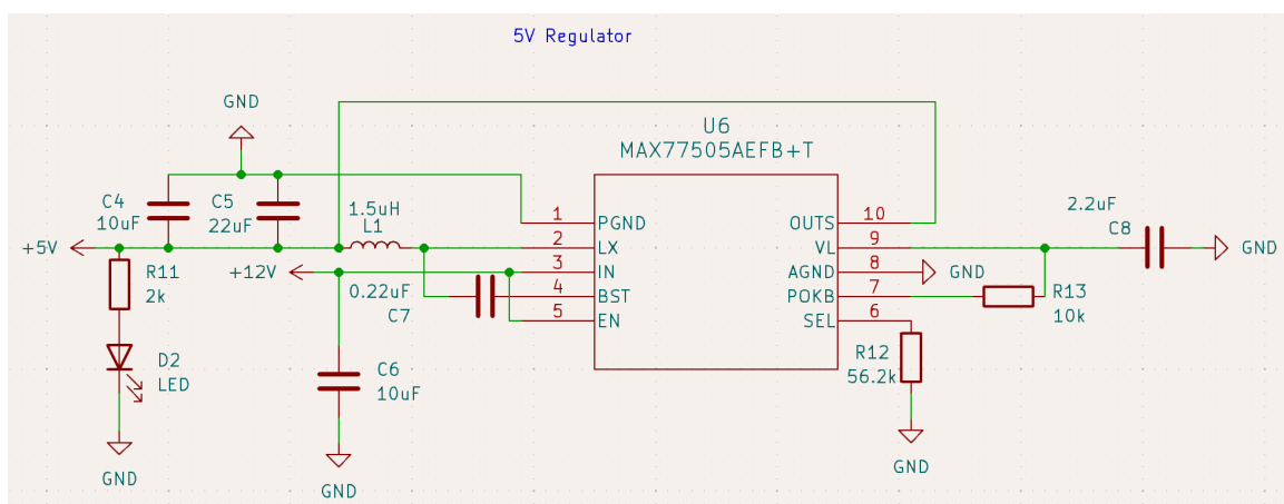
Figure 19: 5V Buck-Converter Schematic
