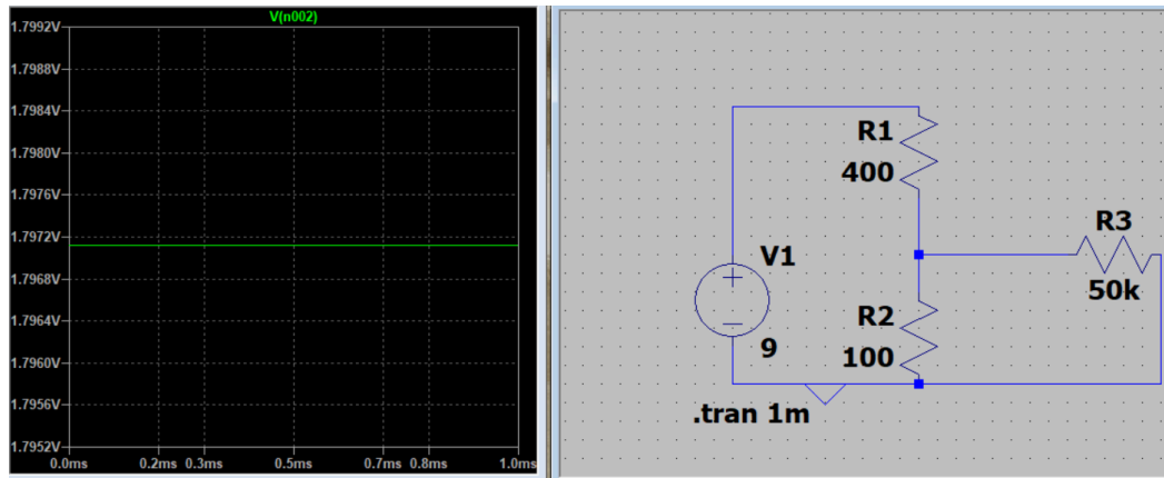
Figure 27: LT-Spice Simulation of Voltage Divider
