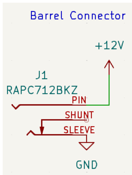
Figure 18: AC-DC Adapter Barrel Connector
