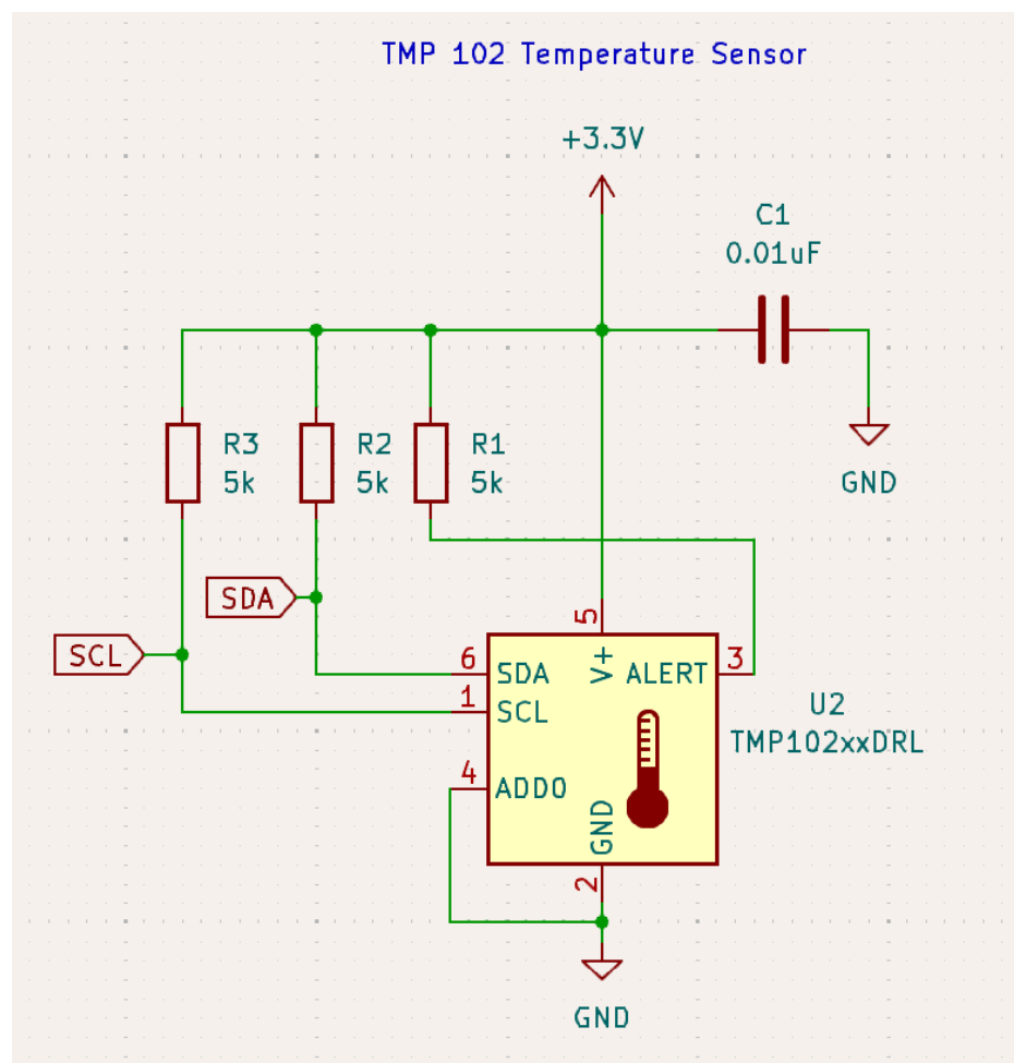
Figure 15: Temperature Sensor Schematic
