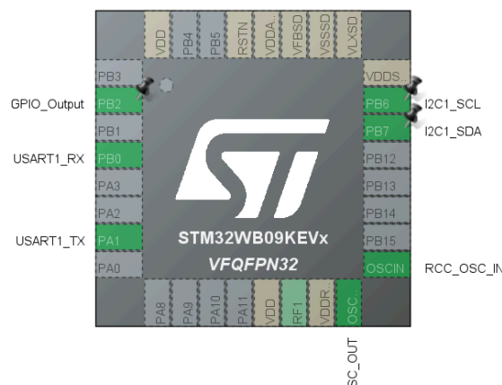
Figure 31: Pinout configuration of the STM32WB09
