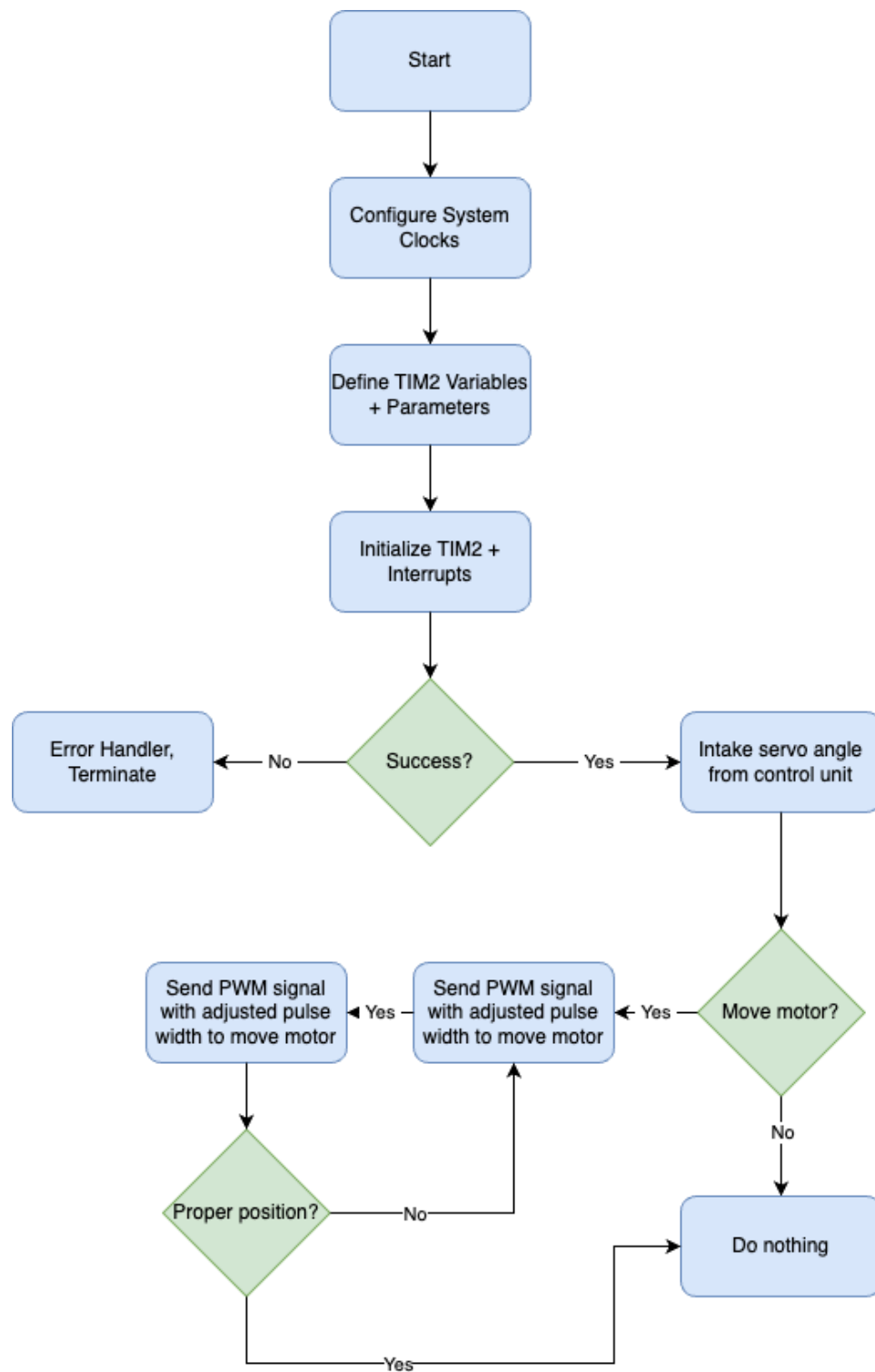
Figure 36: Motor Flowchart
