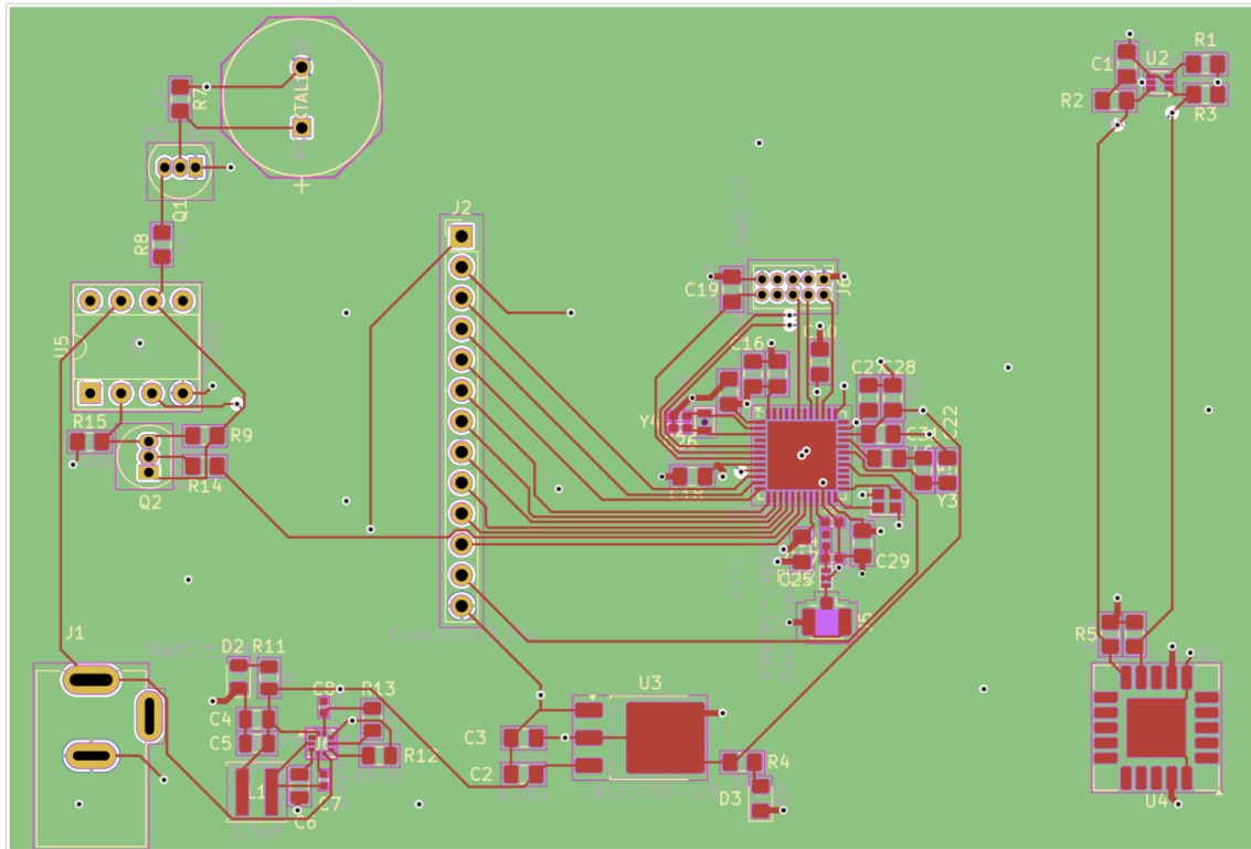
Figure 39: Control unit PCB Layout
