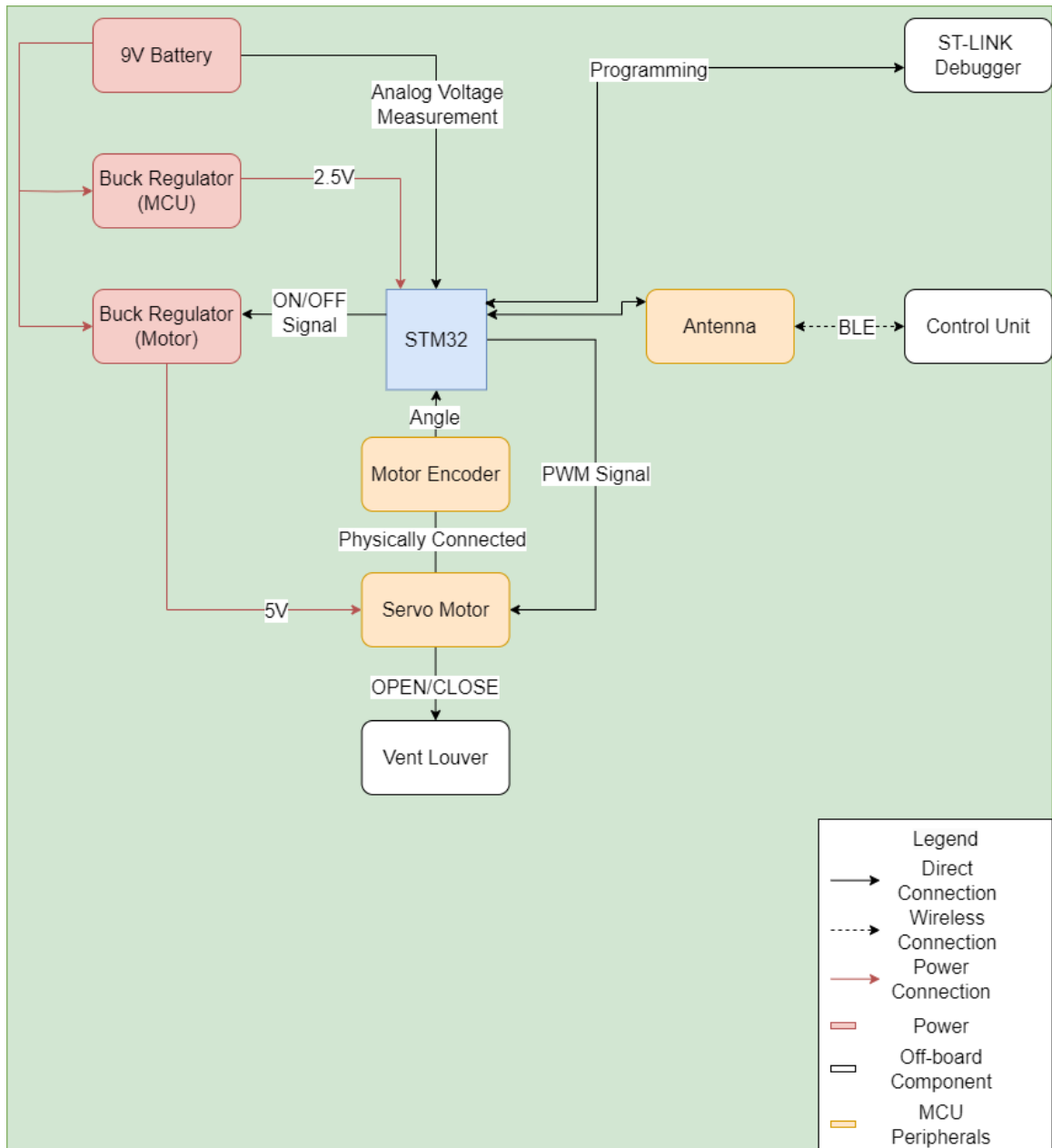
Figure 22: Vent Interaction Subsystem Hardware Block Diagram
