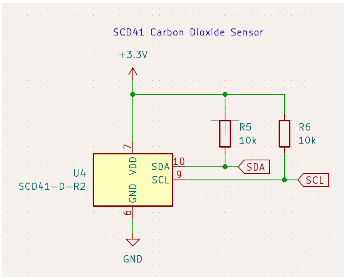
Figure 16: Carbon Dioxide Sensor Schematic
