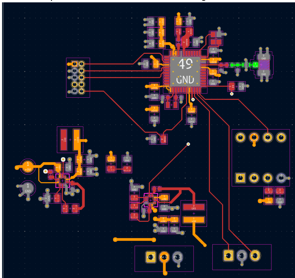
Figure 41: Vent Interaction Subsystem PCB Layout
