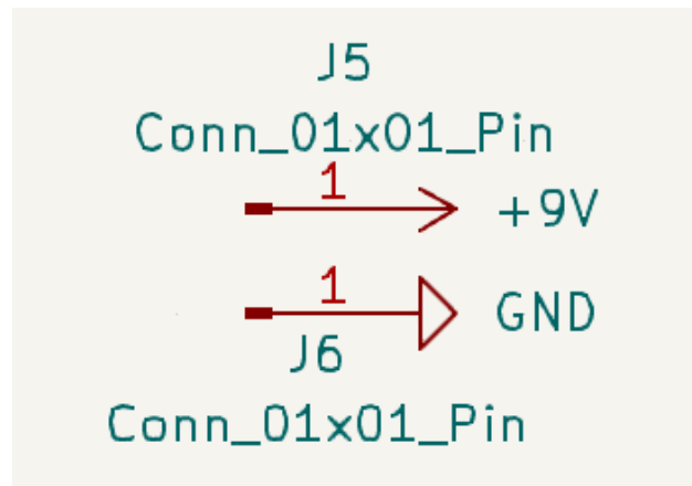
Figure 24: 9V Battery Input Schematic
