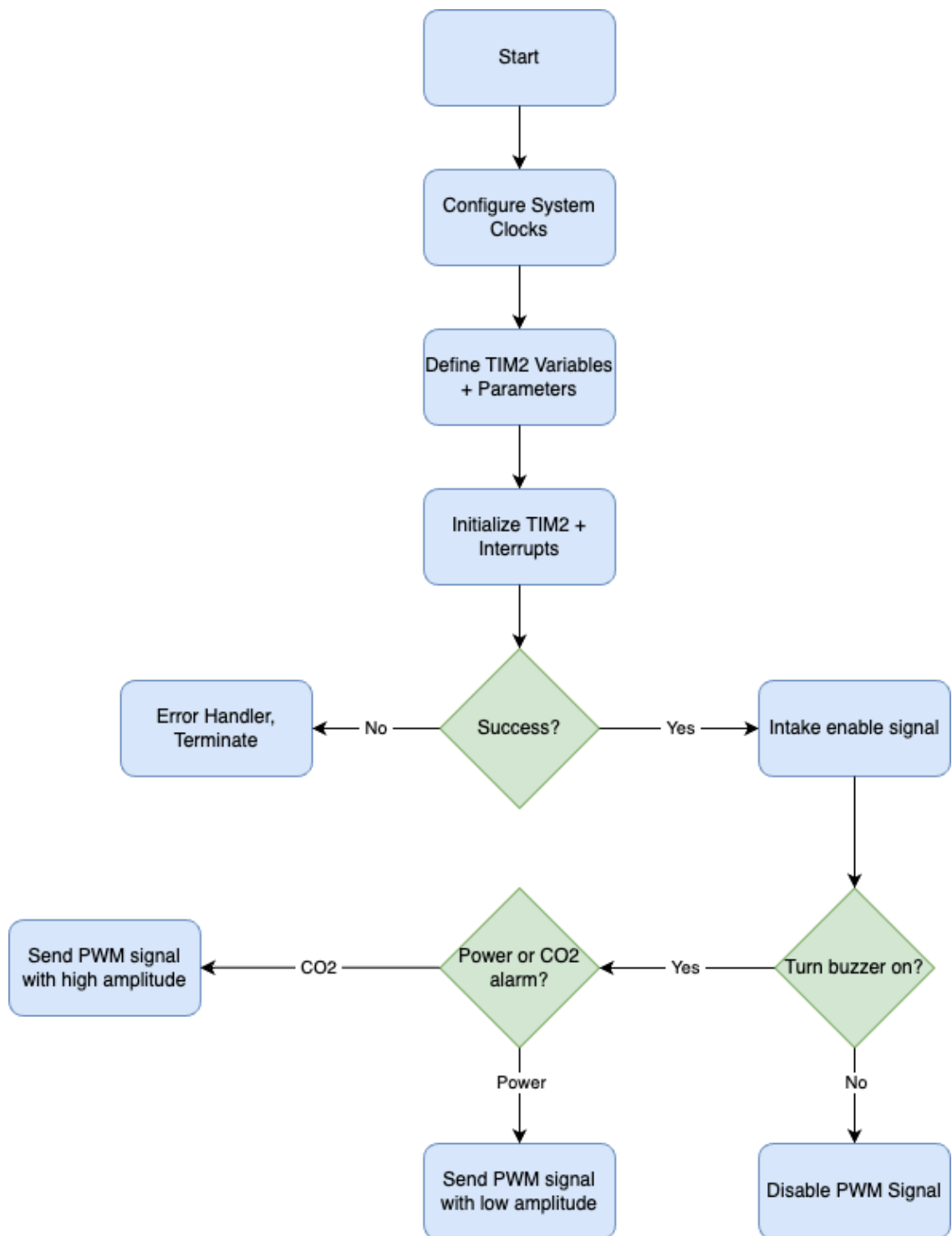
Figure 35: Buzzer Flowchart
