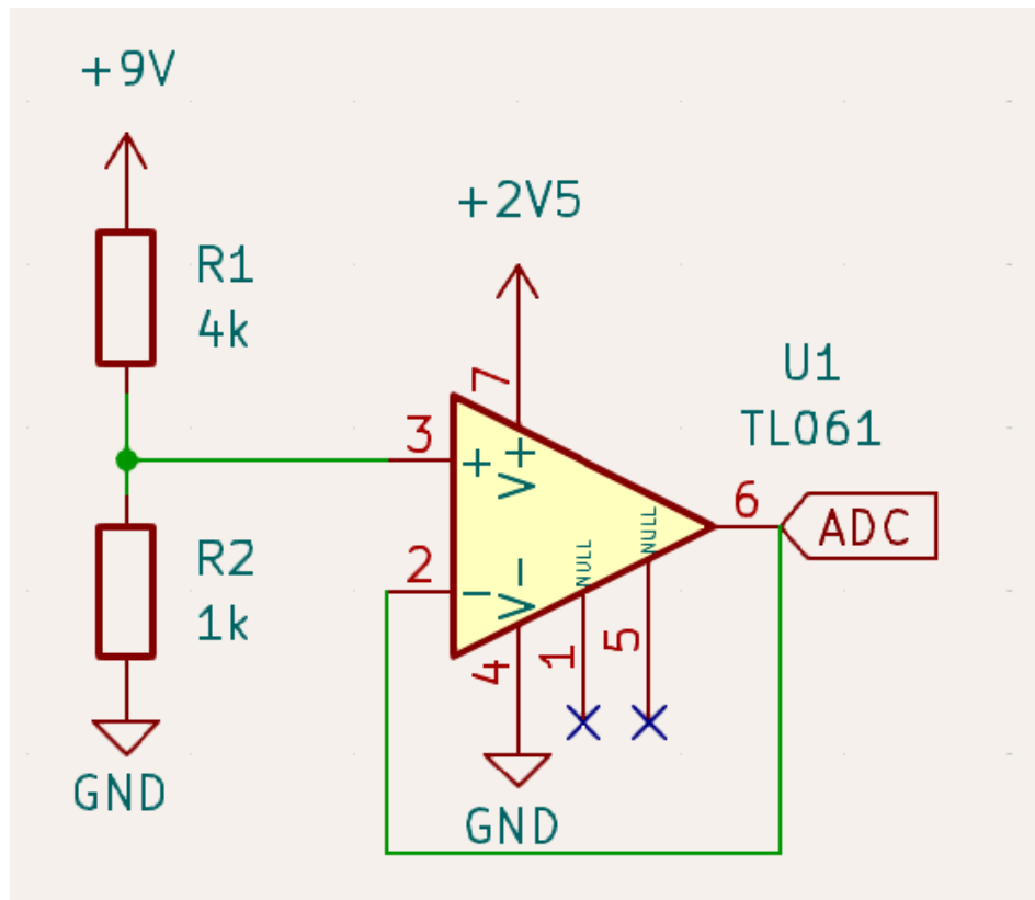
Figure 26: Battery Life Indicator Schematic
