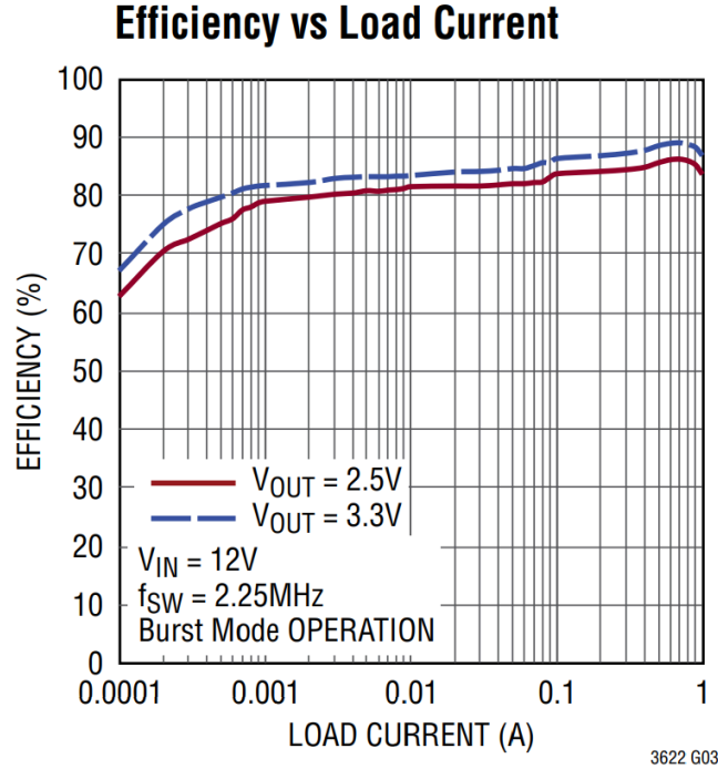
Figure 11: Efficiency vs Load Current of LTC-3622 at 2.5V and 3.3V output [72].
