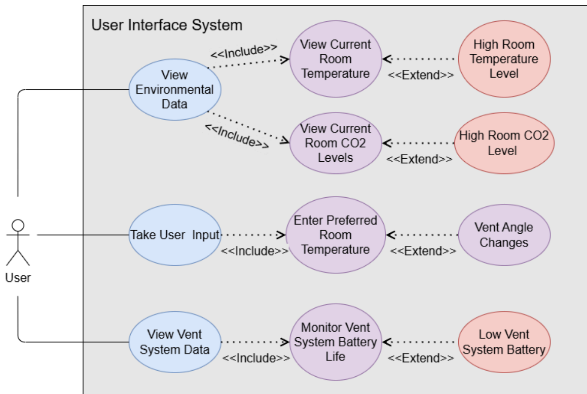
Figure 37: User Interface Use Case Diagram
