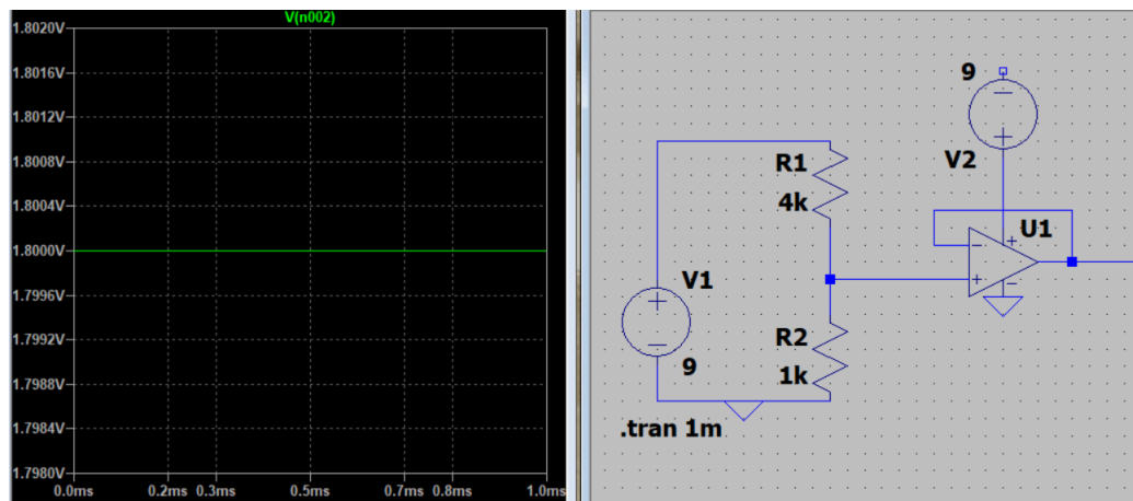
Figure 28: LT-Spice Simulation of Buffered Voltage Divider
