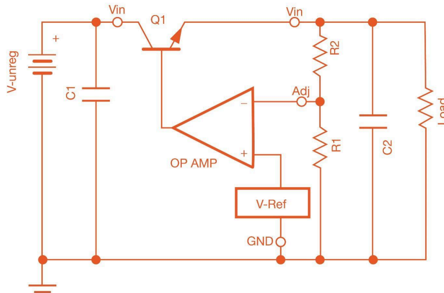
Figure 8: Circuit schematic of simple linear voltage regulator [60].
